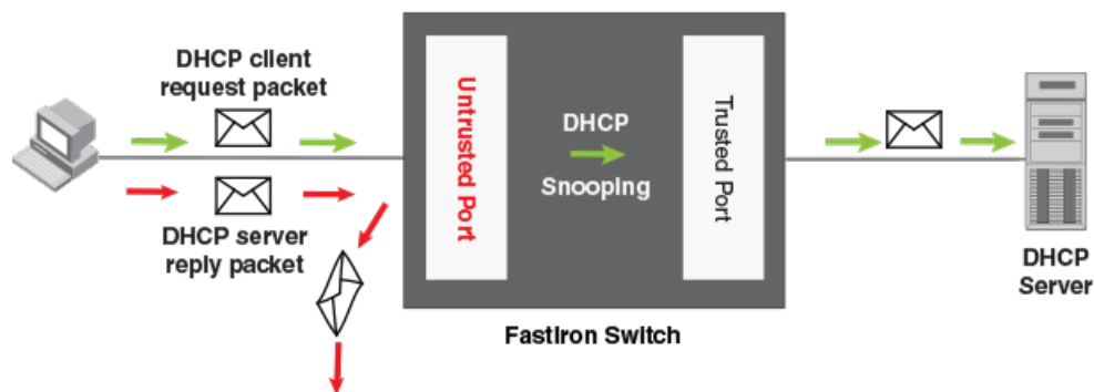
FIGURE 7 DHCP Snooping at Work on an Untrusted Port
